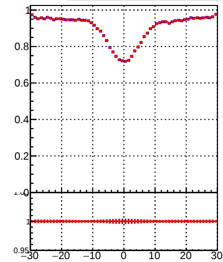
—•— DQM_TT_mkFit-DQM_ —•— DQM_TT_mkFit-DQM_adjusted
