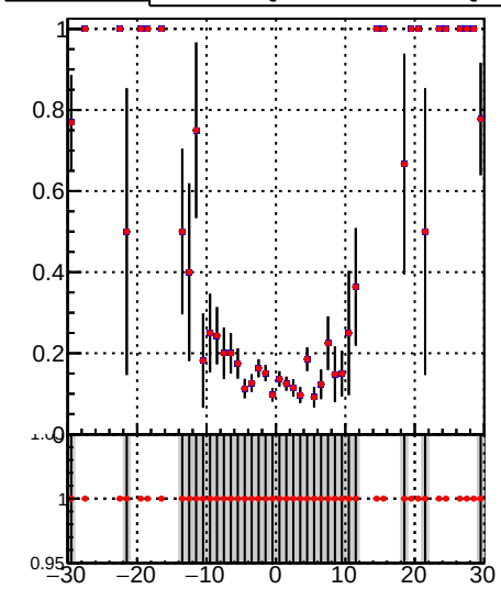
—•— DQM_TT_mkFit-DQM_ —•— DQM_TT_mkFit-DQM_adjusted
