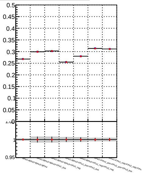
Fake rate vs. DQM_TT_mkFit-DQM DQM_TT_mkFit-DQM_adjusted
