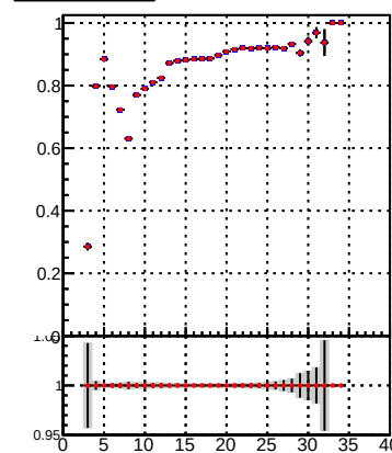
Fake rate vs hit DQM_TT_mkFit-DQM DQM_TT_mkFit-DQM_adjusted
