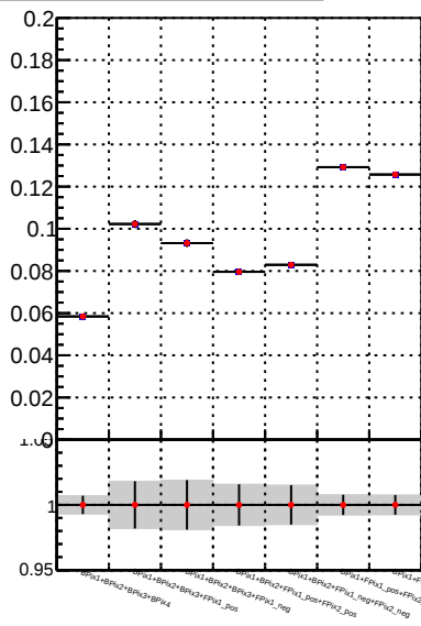
Fake rate vs. —•— DQM TT_mkFit-DQM —•— DQM TT_mkFit-DQM_adjusted
