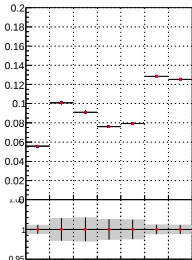
Fake rate vs. DQM TT_mkFit-DQM DQM TT_mkFit-DQM_adjusted
