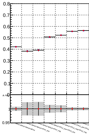
Fake rate vs. DQM TT mkFit-DQM DQM TT mkFit-DQM adjusted
