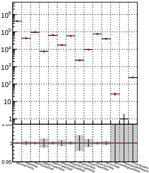
Number —●— DQM_TT_mkFit-DQM_adjusted
