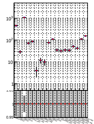
N of reco track vs. \chi^2 (recoToSim) DQM TT mkFit-DQM DQM TT mkFit-DQM_adjusted
