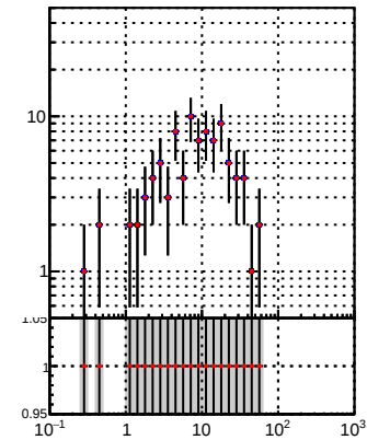
N of reco track vs \eta pT \eta —•— DQM_TT_mkFit-DQM -.-•- DQM_TT_mkFit-DQM_adjusted
