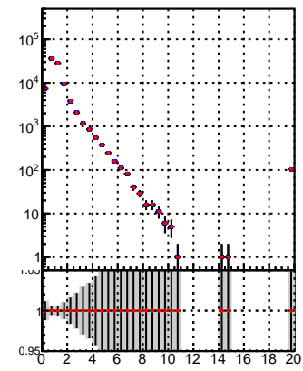
N of reco track vs. \chi^2 for DQM TT and mkFit-DQM adjusted
