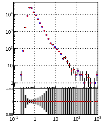
N of reco track vs \eta pT [GeV] —•— DQM_TT_mkFit-DQM_ —•— DQM_TT_mkFit-DQM_ adjusted
