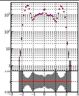
N of reco track vs \eta pT [GeV] —•— DQM_TT_mkFit-DQM_ —•— DQM_TT_mkFit-DQM_ adjusted
