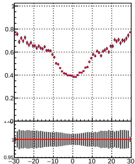
—●— DQM_TT_mkFit-DQM —●— DQM_TT_mkFit-DQM_adjusted
