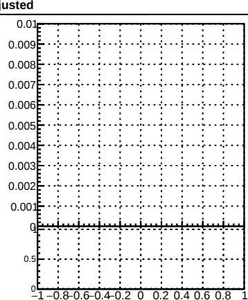
Duplicates Rate vs Dxy(PV)
