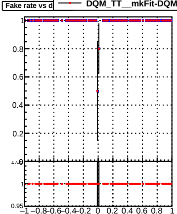
Fake rate vs d
