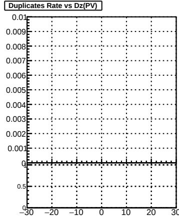
Duplicates Rate vs Dz(PV)
