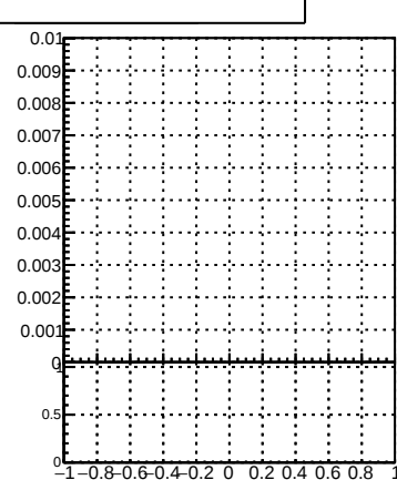
Pileup rate vs dxy(PV)
