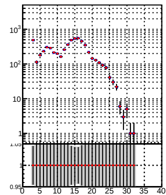
—•— DQM_TT_mkFit-DQM_ —•— DQM_TT_mkFit-DQM_adjusted
