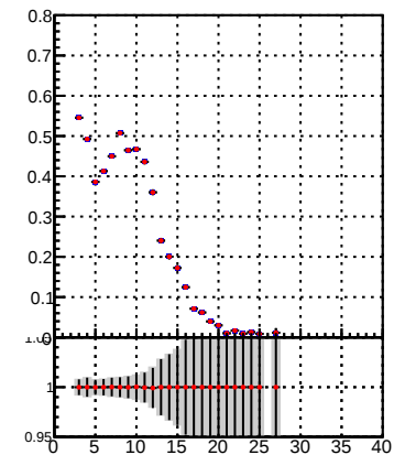
Fake rate vs hit Legend: DQM_TT_mkFit-DQM (blue line with circles), DQM_TT_mkFit-DQM_adjusted (red line with circles)
