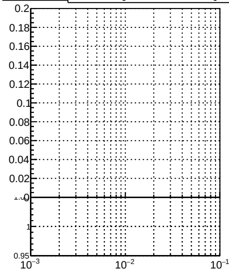
Fake rate vs \epsilon DQM_TT_mkFit-DQM_ DQM_TT_mkFit-DQM_adjusted
