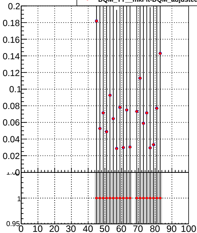
■ DQM_TT_mkFit-DQM_i2 ● DQM_TT_mkFit-DQM_adjustedi2
