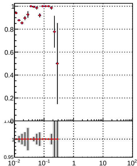
—•— DQM_TT_mkFit-DQM_i2 —•— DQM_TT_mkFit-DQM_adjusted2
