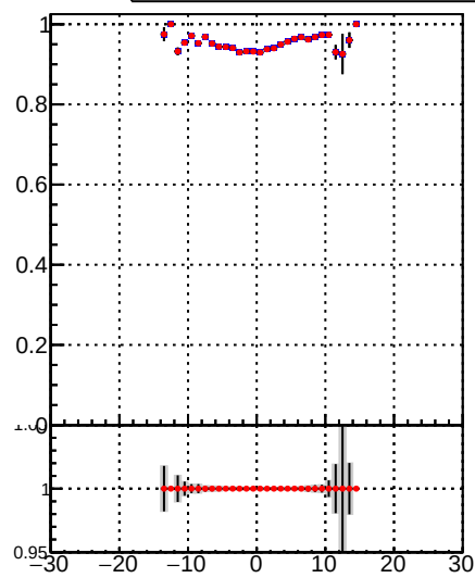
—•— DQM_TT_mkFit-DQM_i2 —•— DQM_TT_mkFit-DQM_adjusted2
