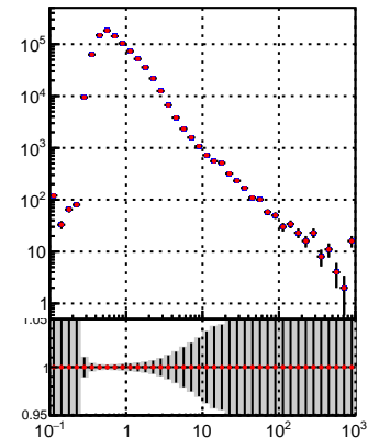
—•— DQM_TT_mkFit-DQM_i2 —•— DQM_TT_mkFit-DQM_adjusted2
