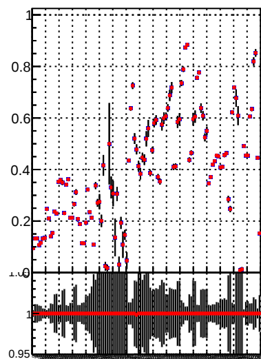
Fake rate vs. DQM TT mkFit-DQM_i2 DQM TT mkFit-DQM_adjustedI2
