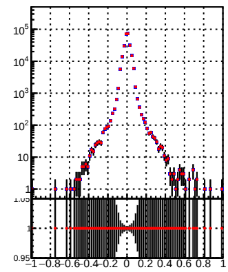
—•— DQM_TT_mkFit-DQM_i2 —•— DQM_TT_mkFit-DQM_adjustedI2
