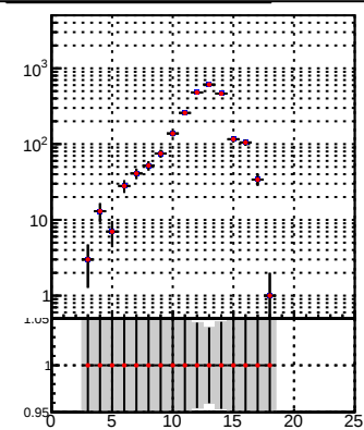
—•— DQM_TT_mkFit-DQM_i2 —•— DQM_TT_mkFit-DQM_adjustedi2
