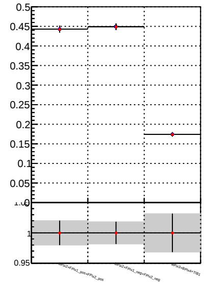
Fake rate vs. DQM_TT_mkFit-DQM_i2 DQM_TT_mkFit-DQM_adjustedi2
