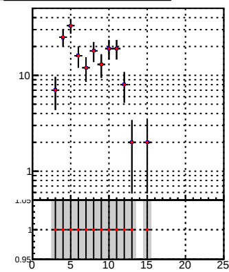
N of associated (recoToSim) duplicate tracks vs i
