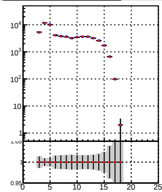
N of associated (recoToSim) tracks vs i
