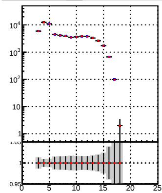
N of reco track vs i
