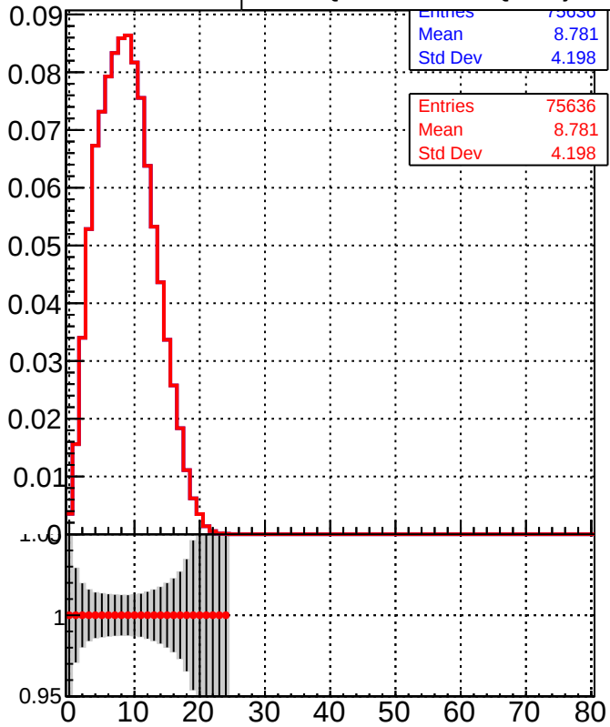
Legend: DQM_TT_mkFit-DQM_i2 (grey histogram), DQM_TT_mkFit-DQM_adjustedi2 (red line with diamonds)
