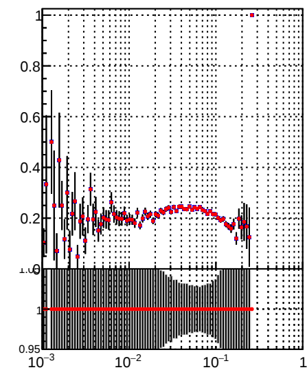
—•— DQM_TT_mkFit-DQM_i2 —•— DQM_TT_mkFit-DQM_adjusted2
