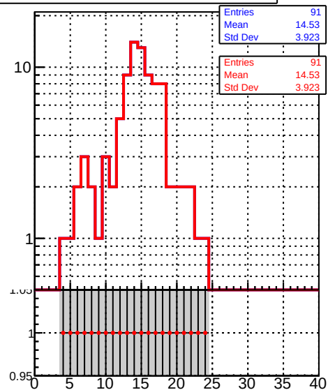
mean hit Legend: DQM_TT_mkFit-DQM_i2 (blue line with dots), DQM_TT_mkFit-DQM_adjusted2 (red line with dots)
