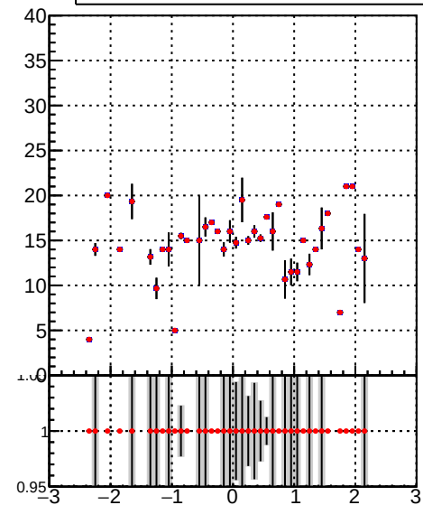
mean hit Legend: DQM_TT_mkFit-DQM_i2 (blue line with dots), DQM_TT_mkFit-DQM_adjusted2 (red line with dots)
