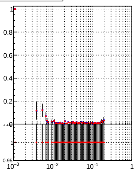
Duplicates Rate vs \sqrt{s}
