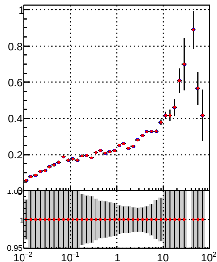
—•— DQM_TT_mkFit-DQM_i2 —•— DQM_TT_mkFit-DQM_adjusted2
