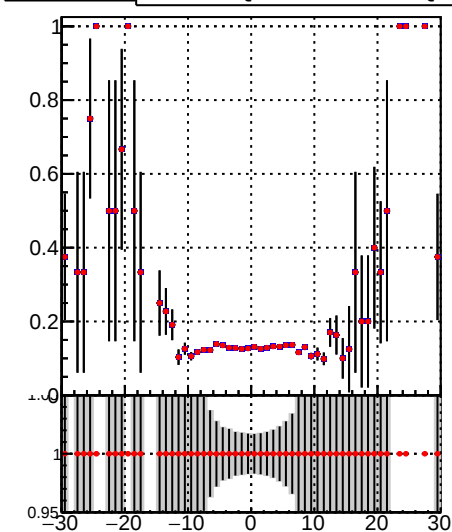
■ DQM_TT_mkFit-DQM_i2 ● DQM_TT_mkFit-DQM_adjusted2
