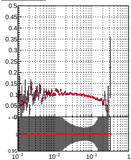
—•— DQM_TT_mkFit-DQM_i2 —•— DQM_TT_mkFit-DQM_adjusted2
