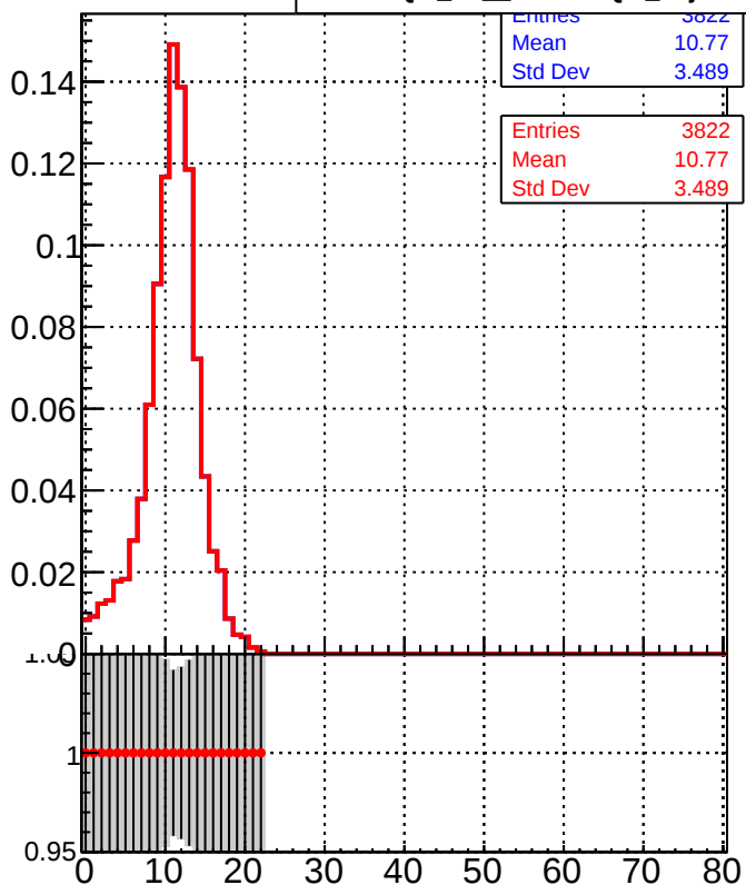
— DQM_TT_mkFit-DQM_i2 — DQM_TT_mkFit-DQM_adjustedI2
