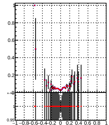
—●— DQM_TT_mkFit-DQM_i2 —●— DQM_TT_mkFit-DQM_adjustedi2
