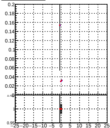
—●— DQM_TT_mkFit-DQM_i2 —●— DQM_TT_mkFit-DQM_adjustedi2
