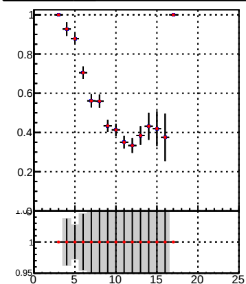
Fake rate vs hit Legend: DQM_TT_mkFit-DQM_i2 (blue line with circles), DQM_TT_mkFit-DQM_adjustedi2 (red line with crosses)
