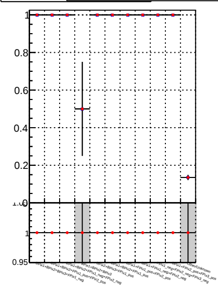
Fake rate vs. — DQM_TT_mkFit-DQM_i2 — DQM_TT_mkFit-DQM_adjustedi2
