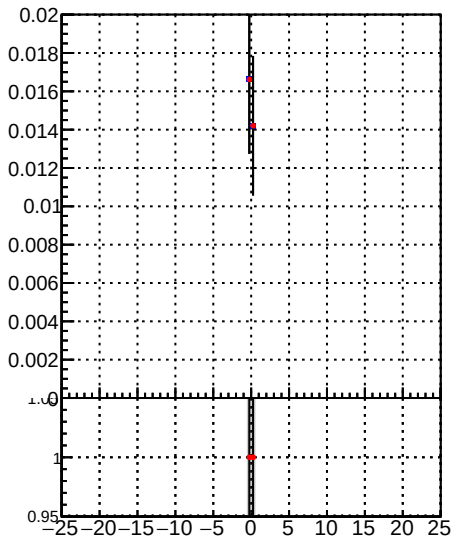
Fake rate vs d —●— DQM TT mkFit-DQM_i2 —●— DQM TT mkFit-DQM_adjustedi2
