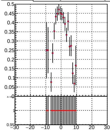
Fake rate vs v_z DQM_TT_mkFit-DQM_i2 DQM_TT_mkFit-DQM_adjustedI2
