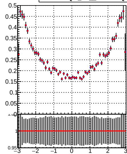
—•— DQM_TT_mkFit-DQM_i2 —•— DQM_TT_mkFit-DQM_adjustedI2
