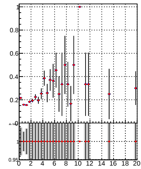
Fake rate vs. — \bullet DQM_TT_mkFit-DQM_i2 — \bullet DQM_TT_mkFit-DQM_adjustedi2
