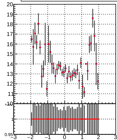
mean hit — DQM_TT_mkFit-DQM_i2 — DQM_TT_mkFit-DQM_adjustedI2
