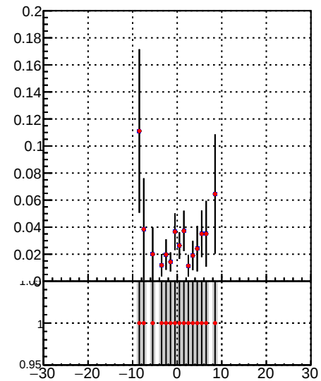
—•— DQM_TT_mkFit-DQM_i2 —•— DQM_TT_mkFit-DQM_adjustedi2
