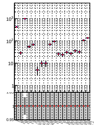
N of reco track vs. \chi^2 (mkFit-DQM_i2 vs mkFit-DQM_adjusted2)
