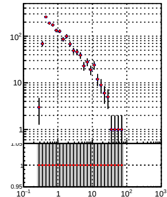
—•— DQM_TT_mkFit-DQM_i2 —•— DQM_TT_mkFit-DQM_adjustedi2
