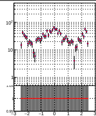
—•— DQM_TT_mkFit-DQM_i2 —•— DQM_TT_mkFit-DQM_adjustedi2
