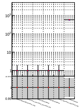
N of reco track vs. \chi^2 — mkFit-DQM_i2 — mkFit-DQM_adjusted2
