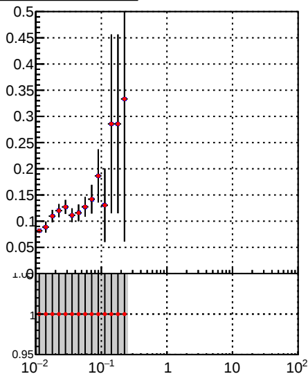
—•— DQM_TT_mkFit-DQM_i2 —•— DQM_TT_mkFit-DQM_adjustedI2
