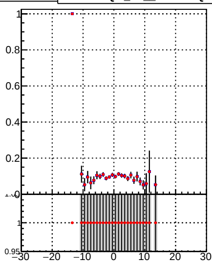
—•— DQM_TT_mkFit-DQM_i2 —•— DQM_TT_mkFit-DQM_adjustedI2
