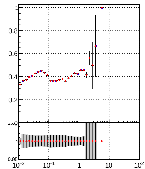
Legend: DQM_TT_mkFit-DQM_i2 DQM_TT_mkFit-DQM_adjusted2
