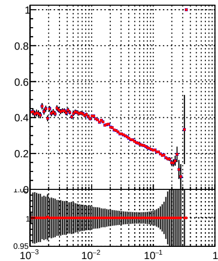
—•— DQM_TT_mkFit-DQM_i2 —•— DQM_TT_mkFit-DQM_adjustedI2
