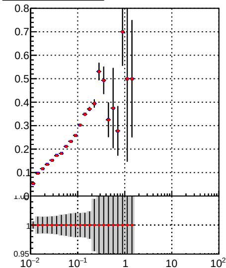
—•— DQM_TT_mkFit-DQM_i2 —•— DQM_TT_mkFit-DQM_adjusted2
