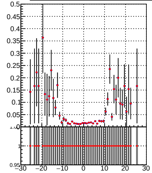
Efficiency vs. sim PV z Legend: ■ DQM_TT_mkFit-DQM_i2 ● DQM_TT_mkFit-DQM_adjusted2
